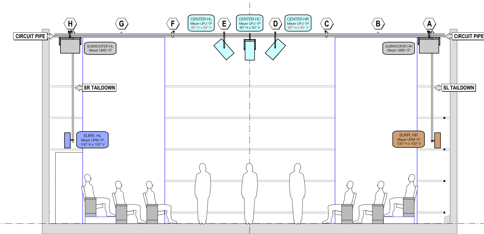
2 Front Elevation
