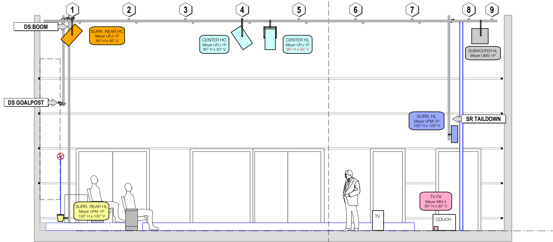
1 SR Section
